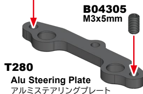
B04305 M3x5mm
