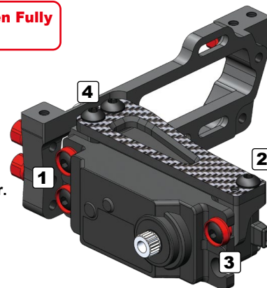
B01306 M3x6mm
