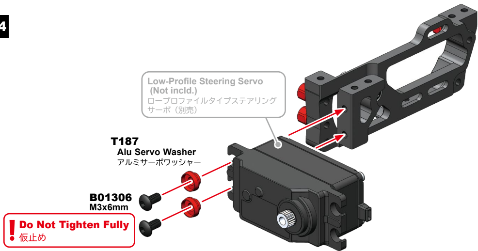
B01306 M3x6mm
