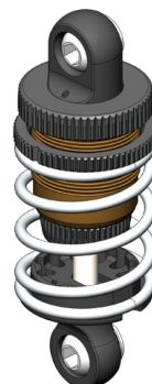
ASSEMBLY VIEW
